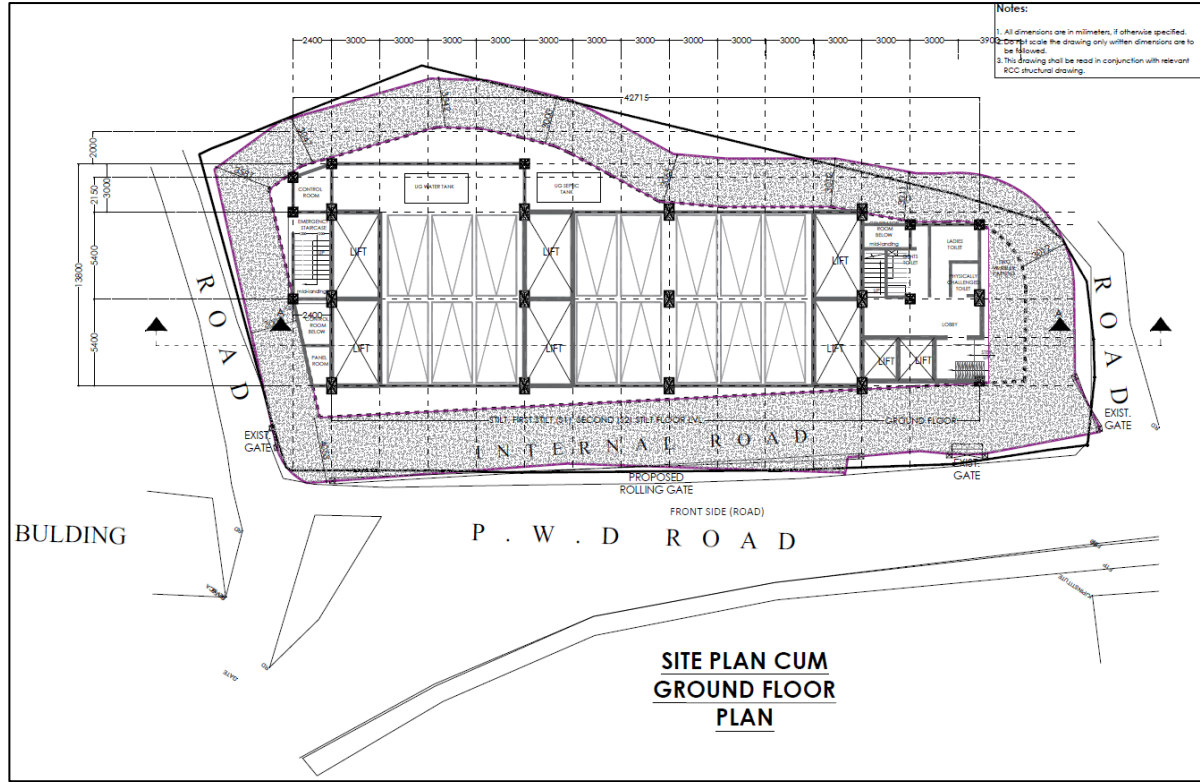
Figure 13: Ground Floor layout plan including Stilt floors
