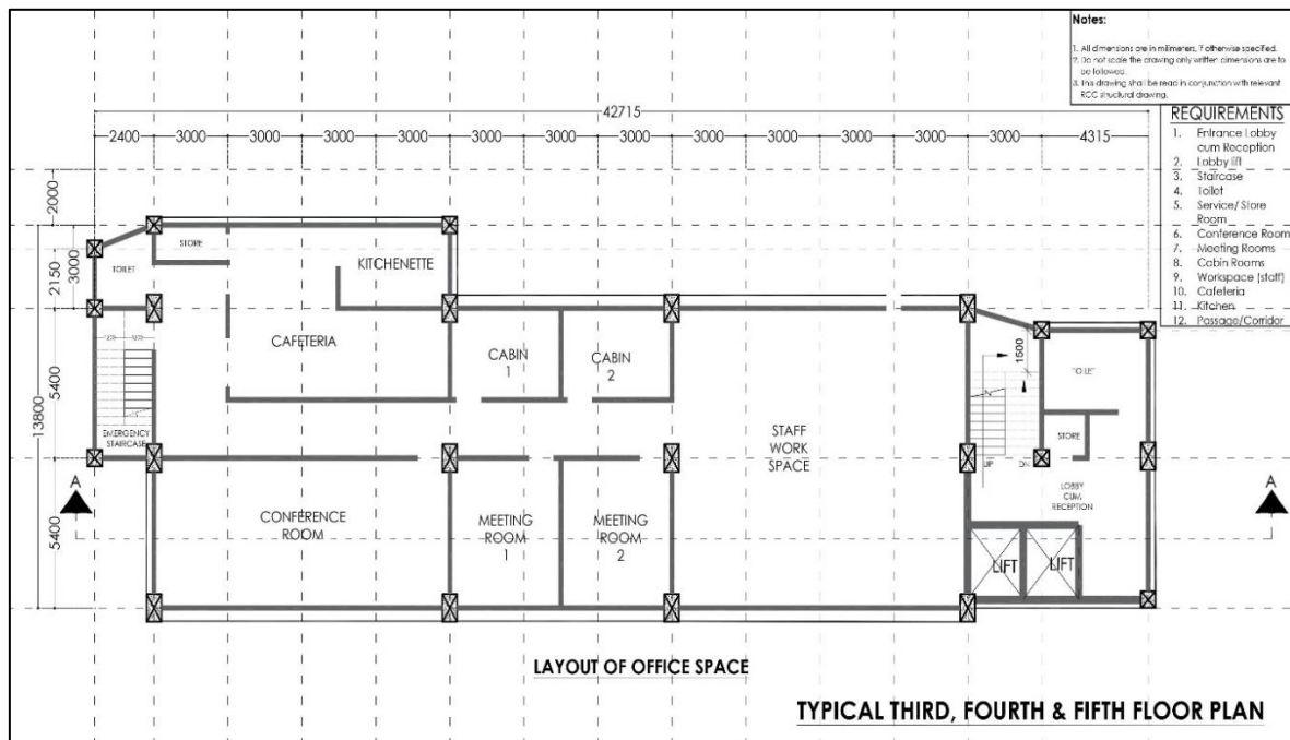
Figure 12: Typical Layout for Office floors
