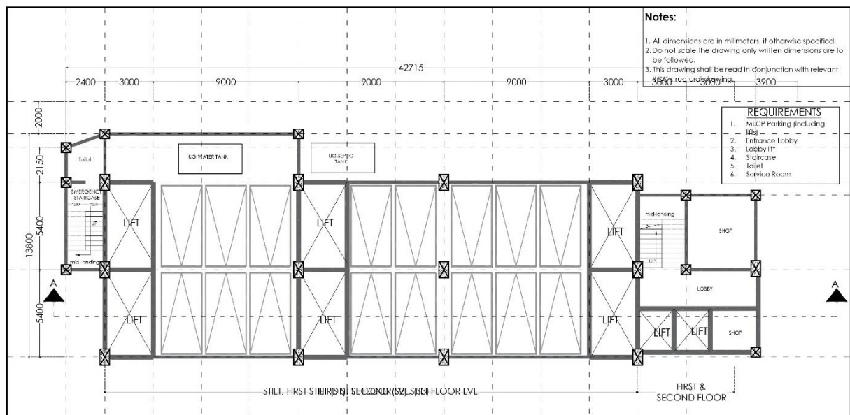
Figure 14: Typical parking layout plan
